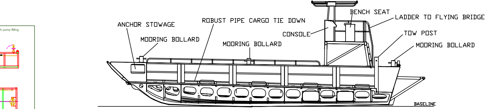
INBOARD PROFILE
